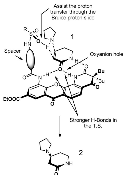
Figure 2. Proposed mechanism for the catalytic effect of the receptors with sulfonamide active groups in the addition of amines to the lactam 1 .
