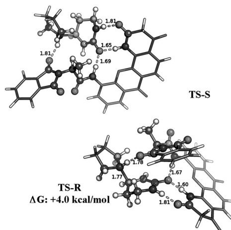
Figure 4. Structure of the transition states obtained from modelling studies for receptor 8 .
