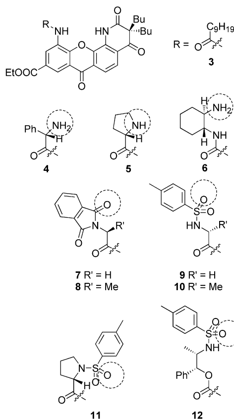
Scheme 1. Structure of the catalysts studied in this work. The group responsible for catalysis by the proton slide is highlighted.
