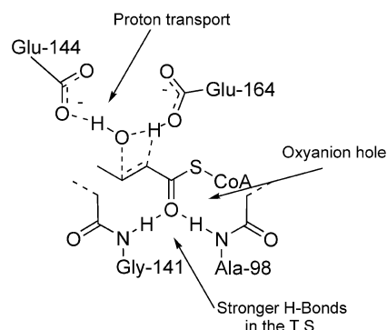
Figure 1. Structure of the oxyanion hole in enoyl-CoA hydratase.
