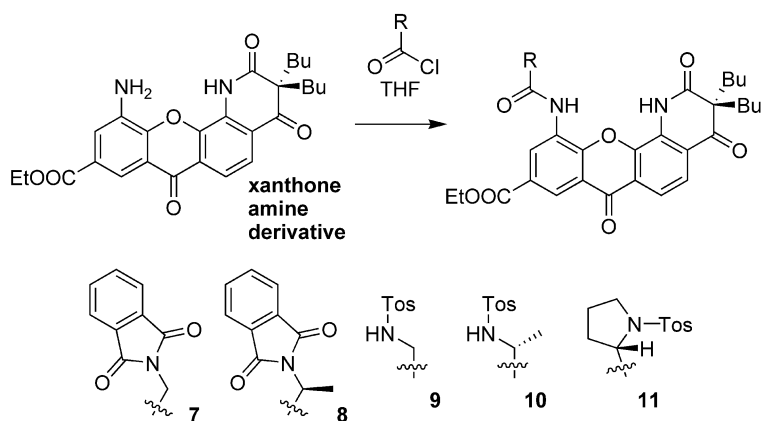
Figure 5. Synthesis of the receptors 7 to 11 .
