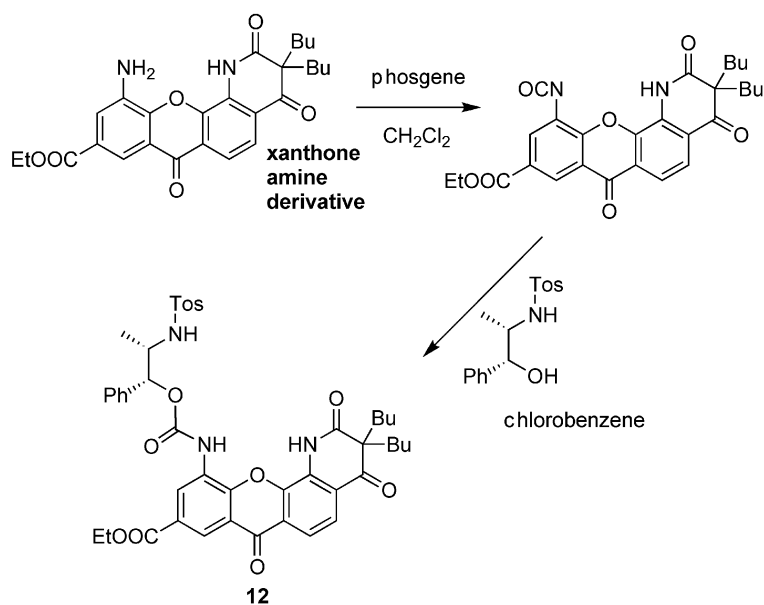
Figure 5. Synthesis of the receptors 7 to 11 .
