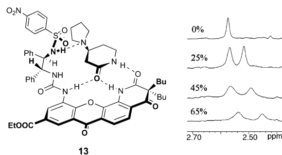
Figure 3. Structure of the complex between the chiral shift reagent 13 and the aminolactam 2 and the induced chemical shifts in the pyrrolidine signals.
